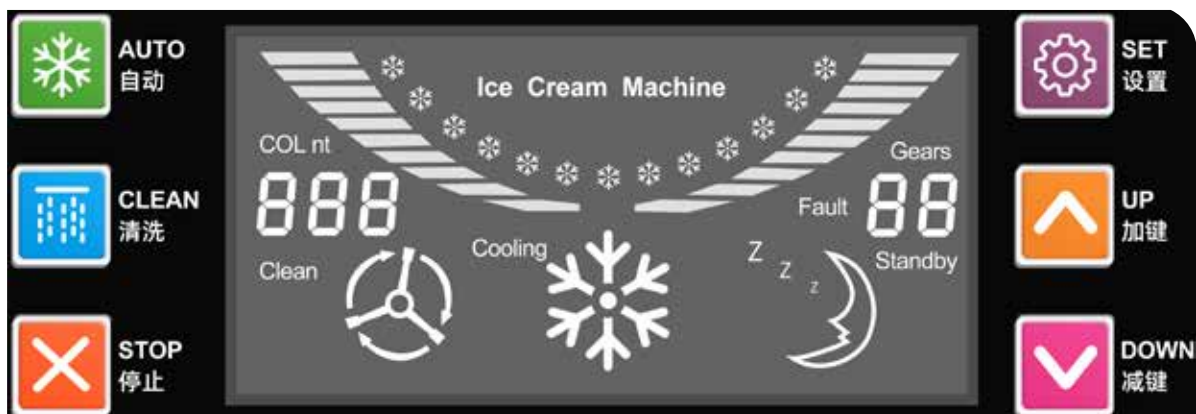
OPERATION PANEL
